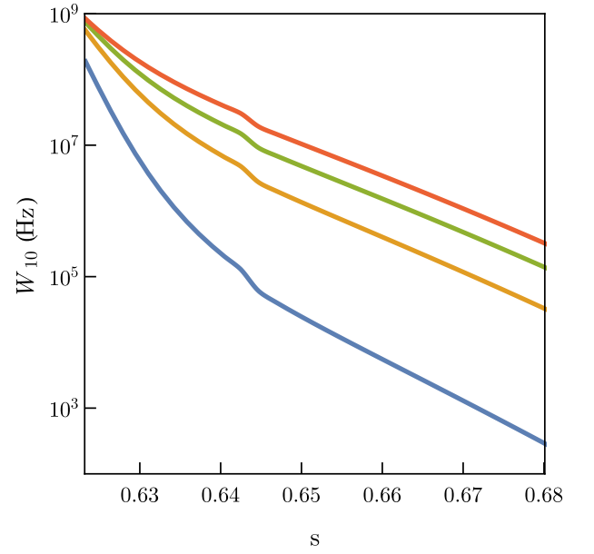
FIG. 10. Logarithmic plots of the transition rate W_{10}(s) vs s after the avoided crossing for different temperatures. Red, green, mustard and blue colors corresponds to T = 12 \text{ mK} , 8 \text{ mK} , 6 \text{ mK} and 4 \text{ mK} respectively. All plots correspond to h_1 = 0.44 and T_{QA} = 20 \mu \text{sec} .
