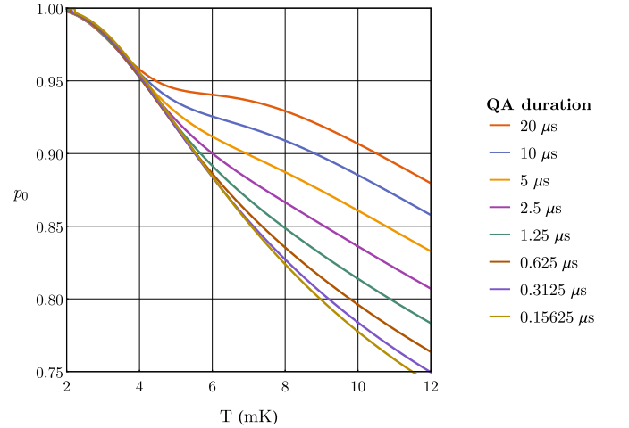
FIG. 11. Success probability of QA p_0 vs T . Different colors corresponds to different duration of the QA process T_{QA} . Plots correspond to h_1 = 0.44 .
